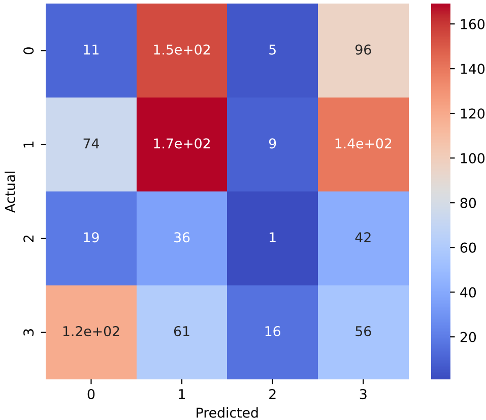
Overall Confusion Matrix OHSS
